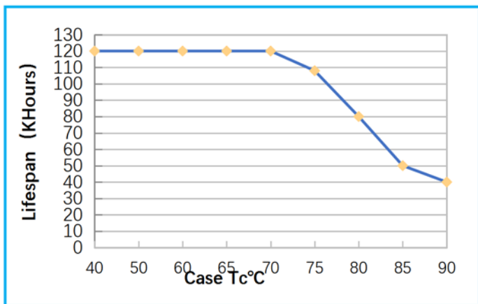
◇ Life-time VS Case Tc°C
