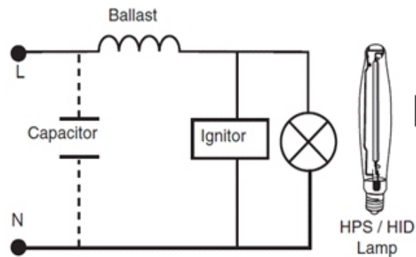
HPS/HID Wiring Diagram
