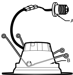
Components Included A. Medium Base Adapter B. Retrofit Assembly C. Instruction Sheet
