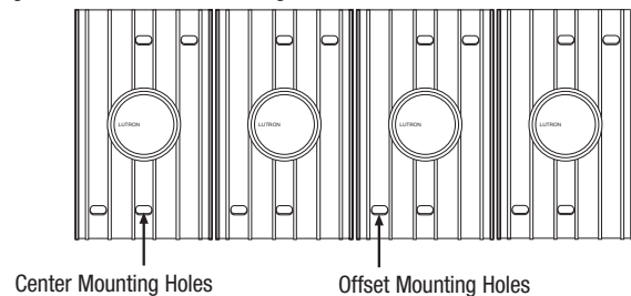
Figure E. Front View - Four-Gang Installation
