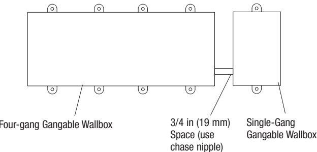
Figure D. Wallbox Positioning Four-Gang Controls
