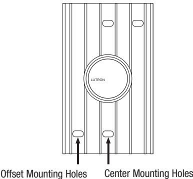
Figure B. Front View - Single Unit Installation
