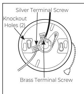
Figure 2. Bottom view of P/N 16502, 16512, and 16526.
