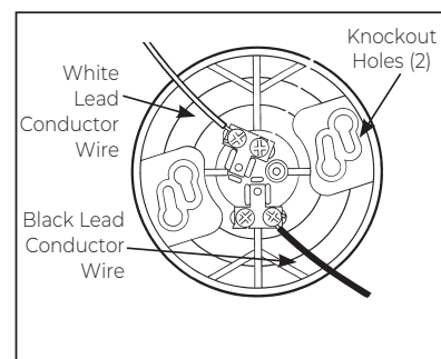
Figure 3. Bottom view of P/N 16520 and 16524.
