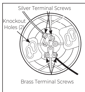
Figure 1. Bottom view of P/N 16500 and 16510.
