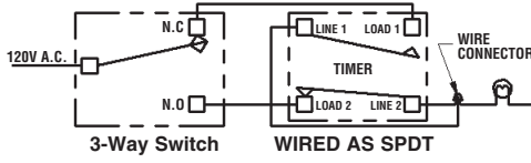
3-Way Switch WIRED AS SPDT
