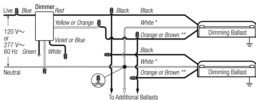
Wiring Diagram 6 Single-Pole Wiring of a 3-Way Control
