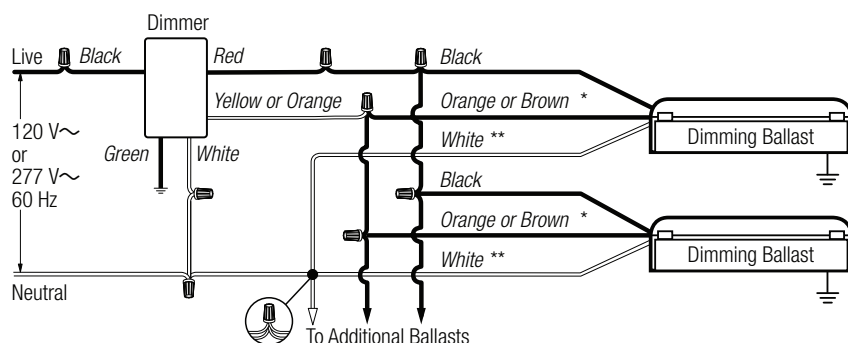
Wiring Diagram 5 Single-Pole Wiring
