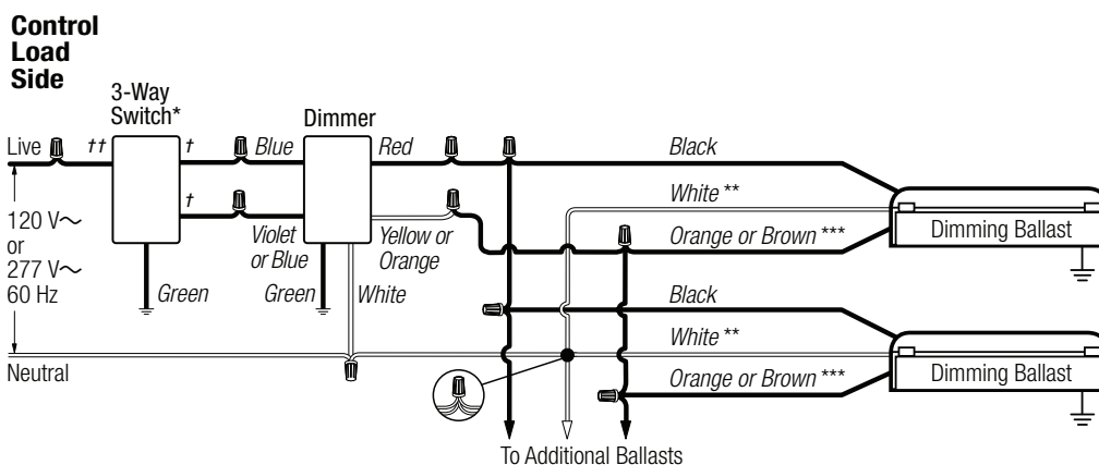
Wiring Diagram 7 3-Way Wiring
