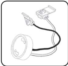
GU-24 Socket Whip (Provided with GU24 units only to convert existing Edison socket fixtures to GU24)
