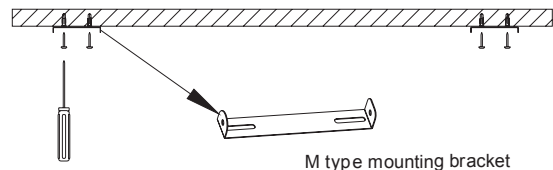
M type mounting bracket
