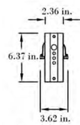
Mounting Arm
