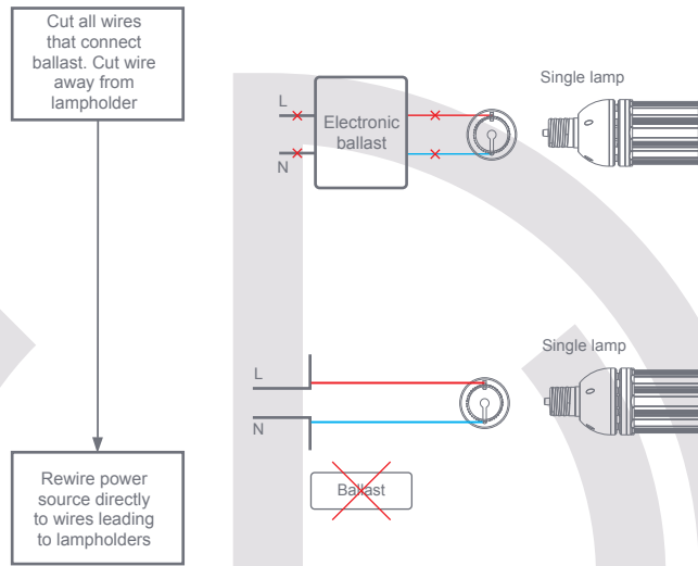
Diagram 2 – Electronic ballast fixture wiring modification
