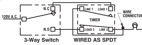
WIRED AS SPDT
