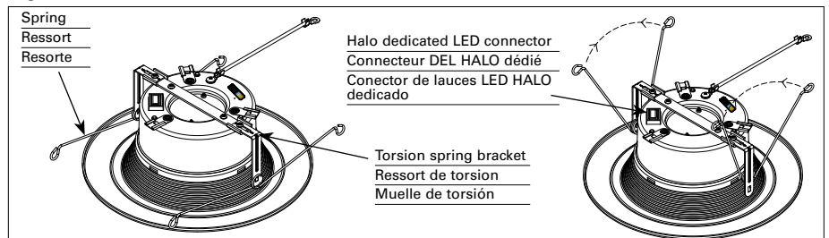
Figure 7. LED Connection
