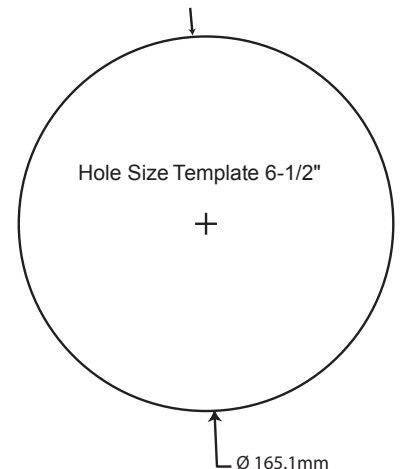
Cutout Dimension
