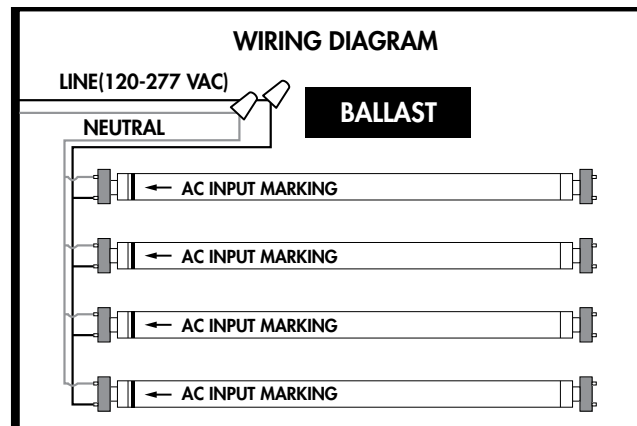
Diagram of fixture with ballast removed.
