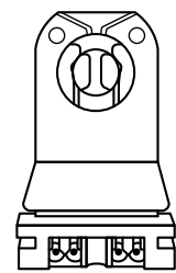
NON-SHUNTED (CORRECT)
