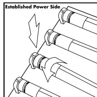
Install ballast cover. Install LiberaT5 lamps, ensuring power end is installed on "power" side of fixture.
