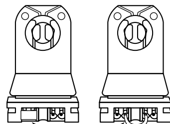
SHUNTED (INCORRECT)
