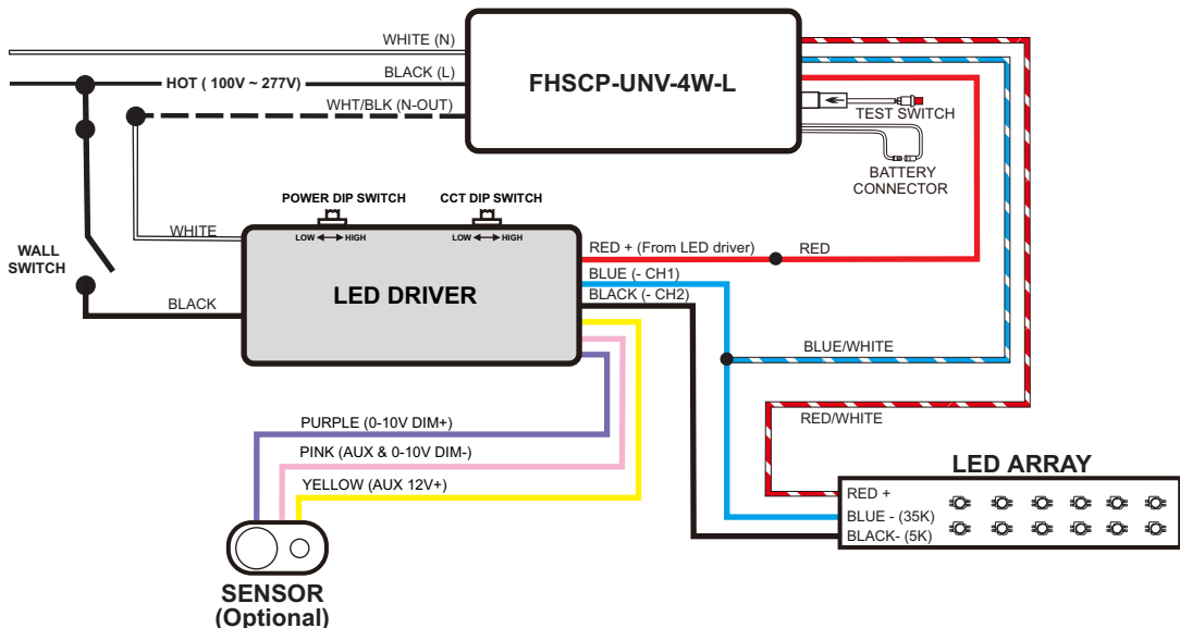
Wiring Diagram 1: 3500K Emergency Output
